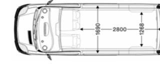
Vivaro DoubleCab L2 H11
