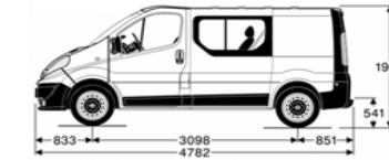
Vivaro DoubleCab L1 H11
