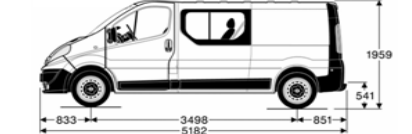
Vivaro DoubleCab L2 H11
